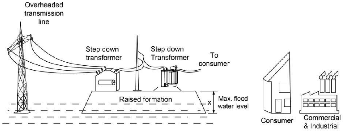
Figure : Substation on raised formation in water logging areas.
