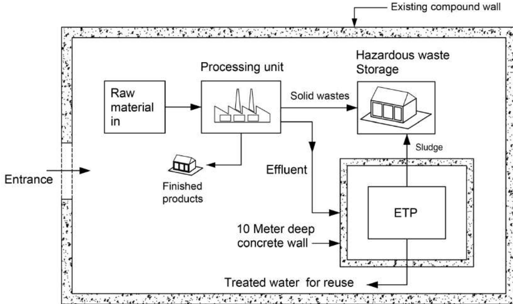
Figure : Effluent discharge control - Measure to control surface & sub surface pollution due to overflow of effluent from leather factory. A deep barrier wall around the ETP will avoid spill over of effluents from the plant. (A partially fool proof method).
