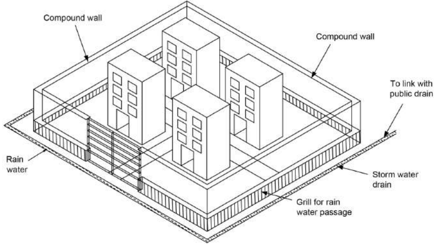
Figure 2 : Gated community - Proposed ways to drain rainwater. (Grill or Porous compound wall for water passage or Storm water drain is to be provided)
