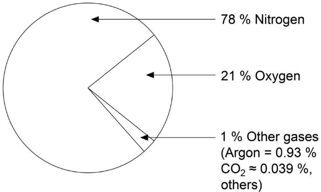
Figure : Composition of atmospheric air (On volume basis).
